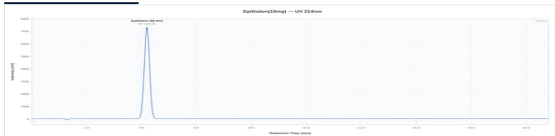
Epitalon 10mg - 04-2606: UV Chromatogram
