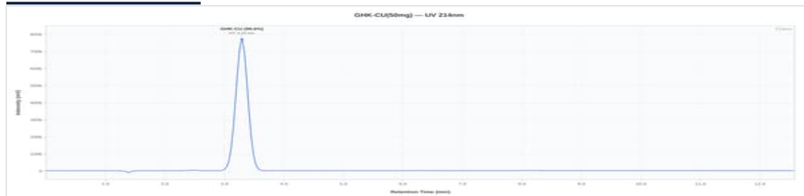
GHK-CU 50mg - 03-2606: UV Chromatogram
