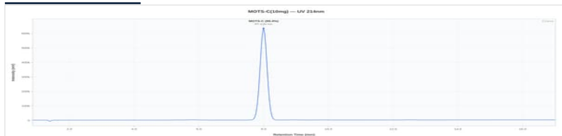
MOTS-C 10mg - 05-606: UV Chromatogram
