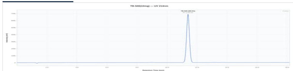
TB-500 10mg - 02-2606: UV Chromatogram
